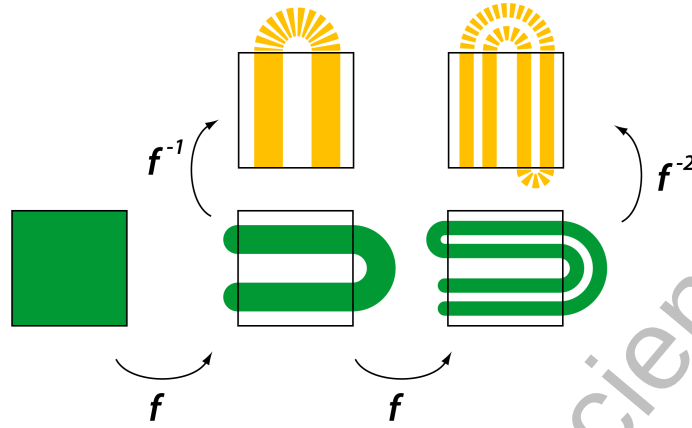
Figure 1: A geometric illustration of the Smale Horseshoe map. The map f stretches, contracts, and folds a square, while the inverse map f^{-1} performs the reverse operation, revealing the fractal structure. (Credit: XaosBits, licensed under FAL. Source: Wikimedia Commons, https://commons.wikimedia.org/w/index.php?curid=9034592 )
